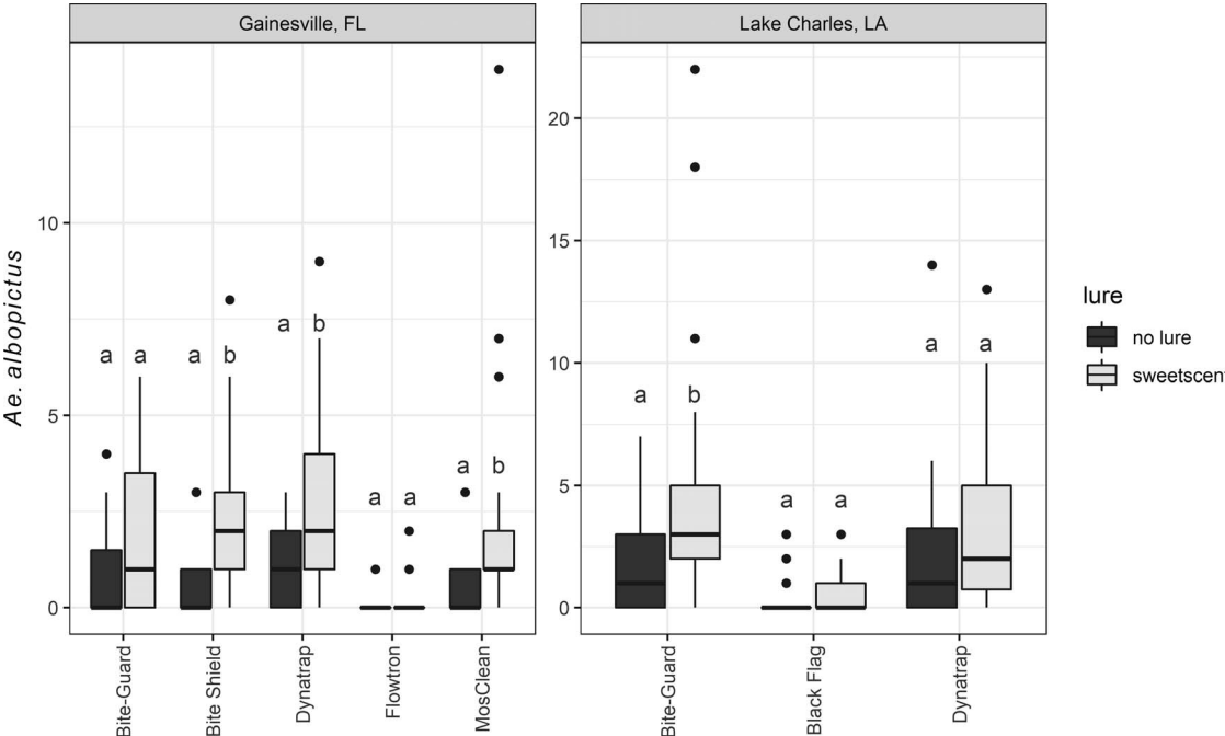
Fig. 1. Boxplots of Aedes albopictus (female and male) catches in several traps with and without BG-Sweetscent in Gainesville, FL, and Lake Charles, LA. Different letters indicate significant different catch rates of the same trap used with or without BG-Sweetscent lure.
