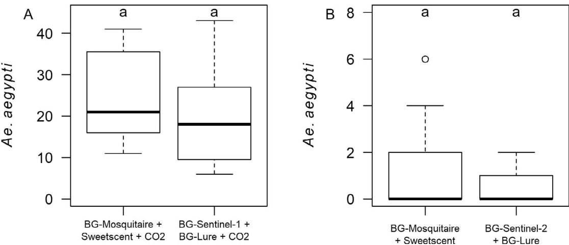
Fig. 2. Boxplots of Aedes aegypti (female and male) catches in BG-Mosquitaire and BG-Sentinel traps (A) in Clovis, CA, and (B) New Orleans. The same letters indicate insignificant different catch rates.
