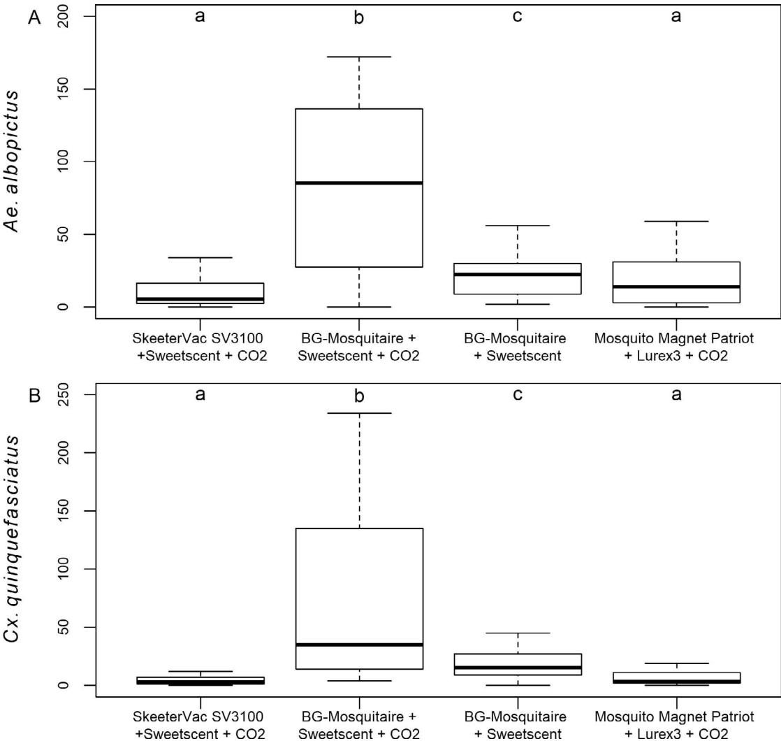
Fig. 3. Boxplots of (A) Aedes albopictus (female and male) and (B) Culex quinquefasciatus catches in 4 different mosquito traps in Lake Charles, LA. Please note that in Fig. 3A, 2 outliers (302 and 523 Ae. albopictus in the BG-Mosquitaire + Sweetscent + CO 2 ) are not shown in order to facilitate visual comparison between boxes. Different letters indicate significantly different catch rates.
