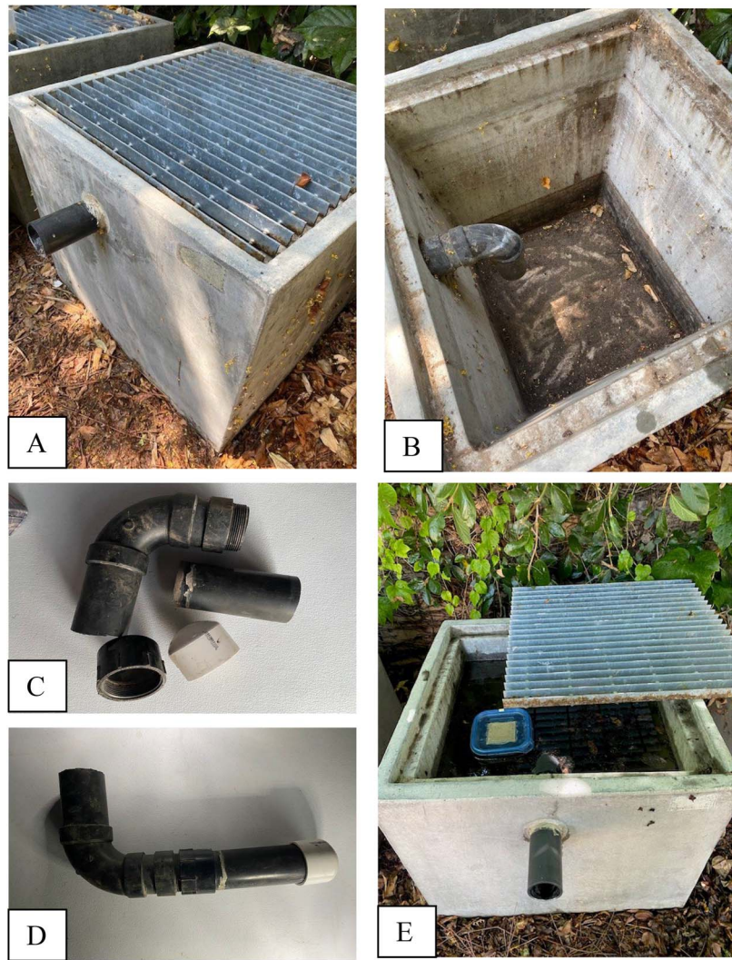
Fig. 2. Cast concrete simulated catch basin: exterior overview (A), interior overview (B), drainpipe components (C), assembled drainpipe (D), and basin in operation (E).
